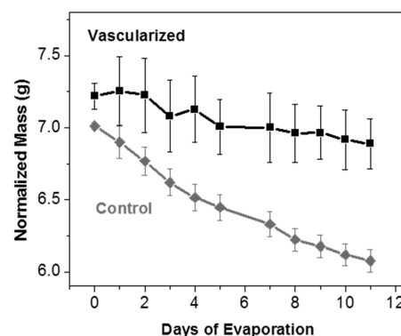
Figure 2. Mass of saturated lubricant-infused PDMS samples containing an embedded vascular network (squares) versus a sample with no vascular network (diamonds) kept at 70 ^{\circ}\text{C} for 11 days. The data were normalized to the dry mass of the samples and error bars represent standard deviation. The control lost mass because of lubricant evaporation more rapidly than the channel system in this accelerated test.
